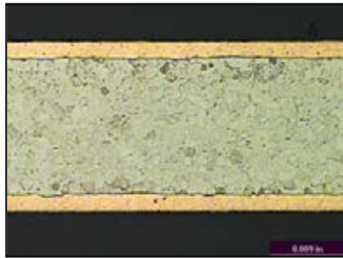
Photomicrograph of CopperPlus (100X)
