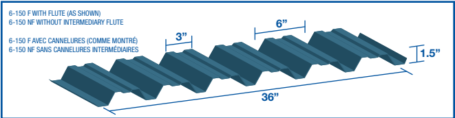
7/8" CORRUGATED | Corrugé 7/8"
